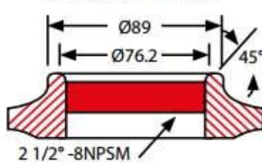
Detail 2 1/2° Thread
